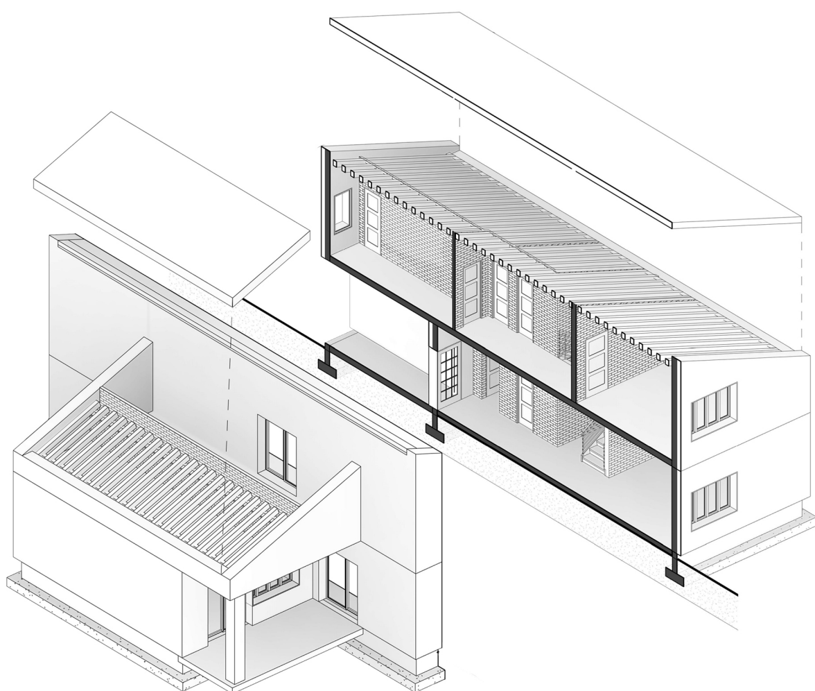
3D presek 3-3
