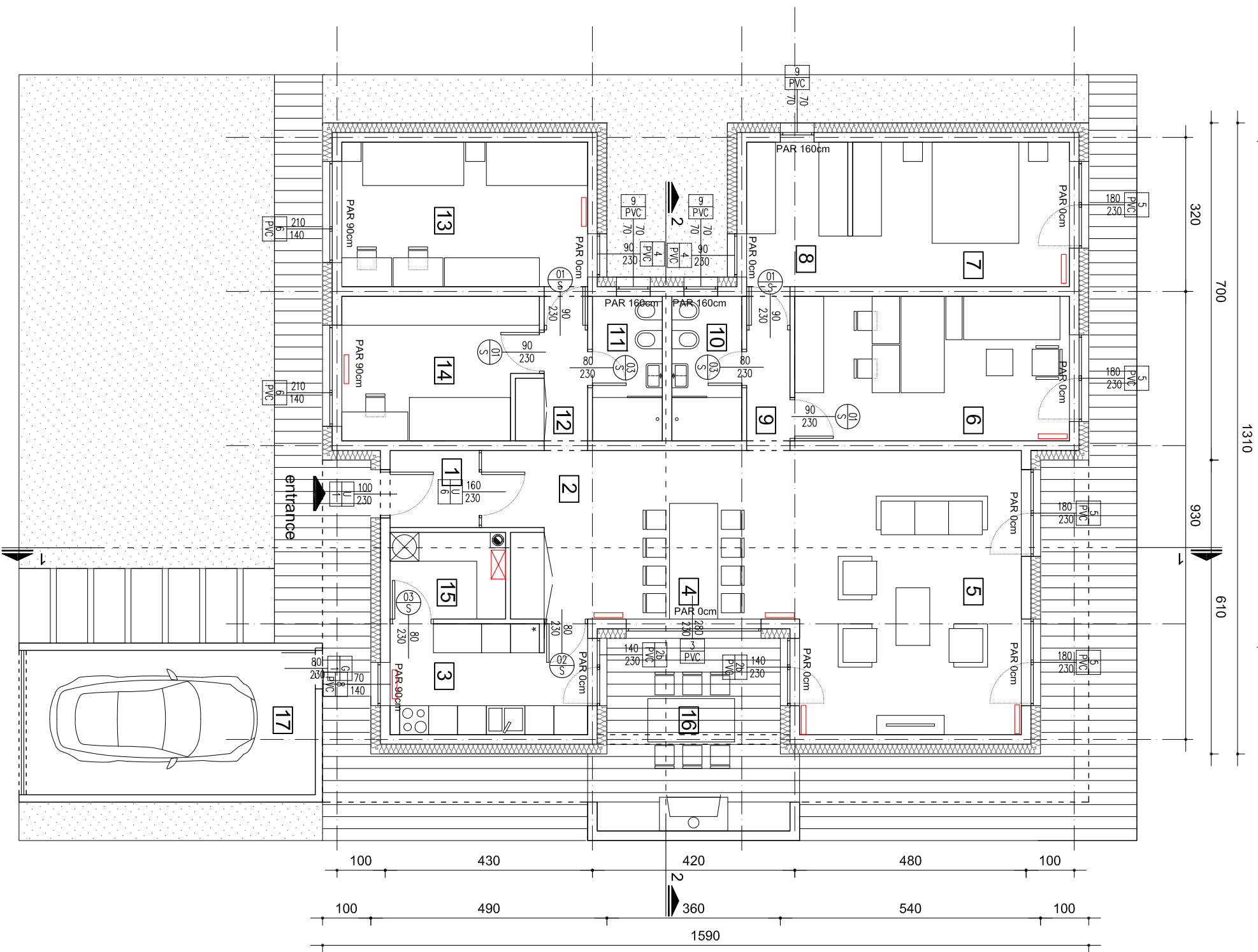
FLOORPLAN
