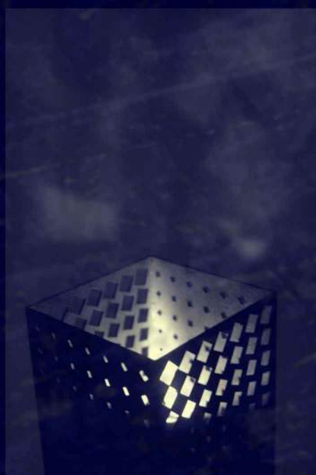
GRASSHOPPER DEFINICIJA
