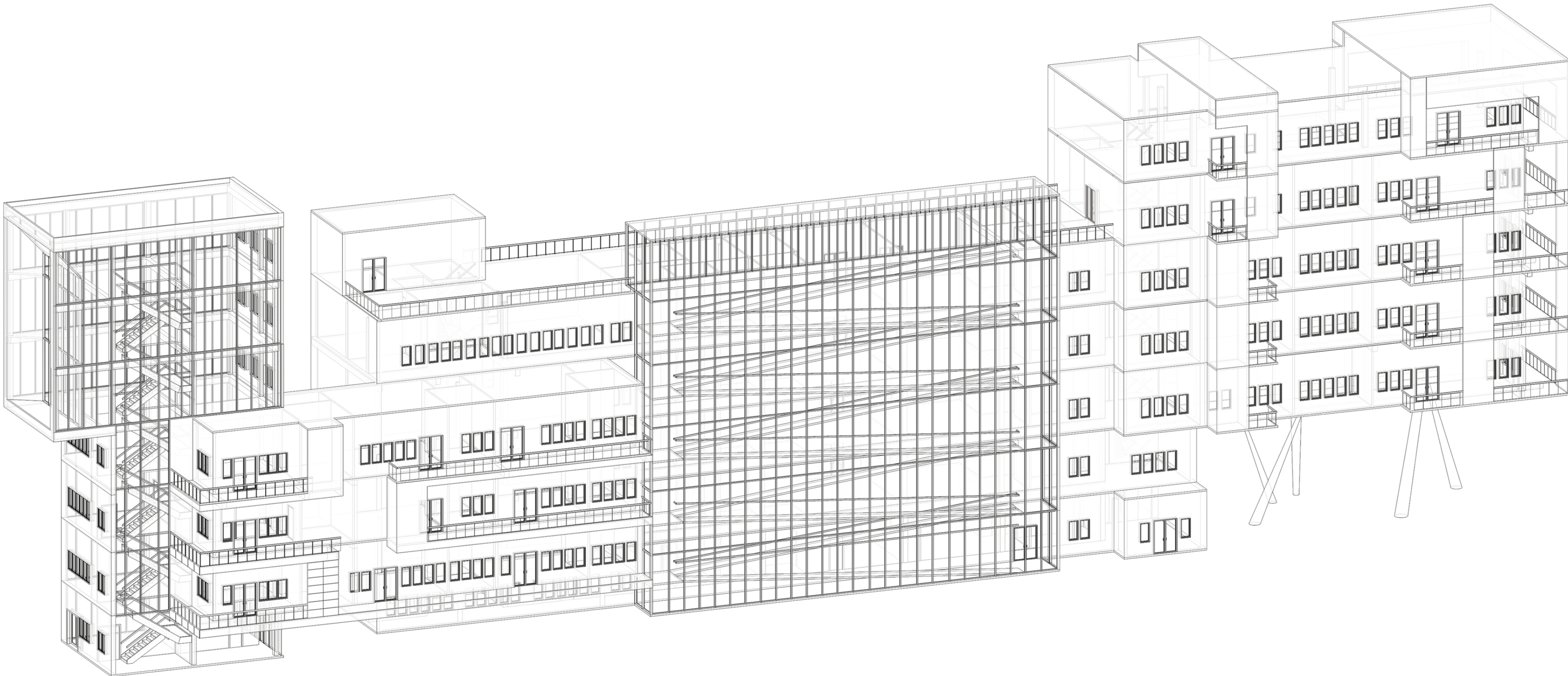
picture No.6 axonometric view
