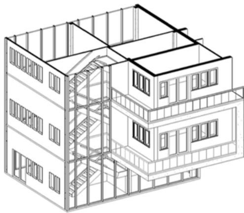
prikaz dela objekta_3d view_section box hidden lines_changed cut view properties
