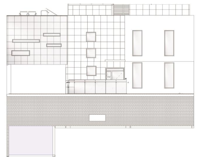
picture No.7 North facade
