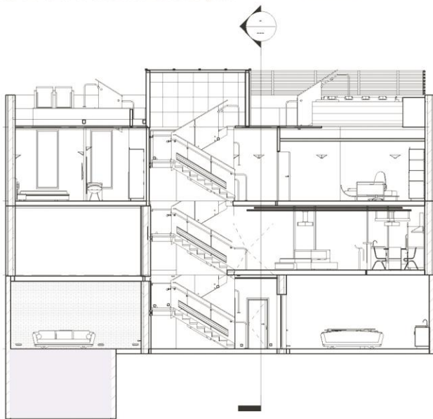
picture No.5 Section 1-1
