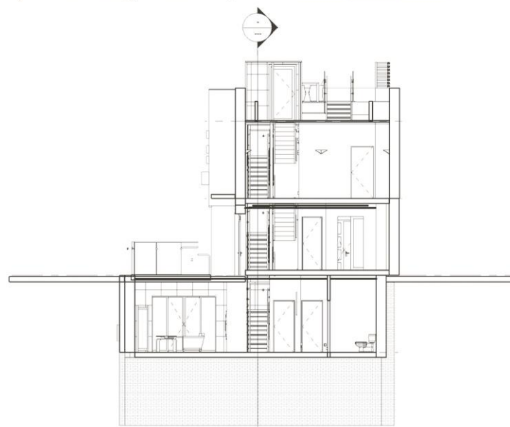
picture No.6 Section 2-2
