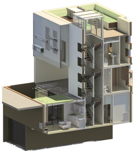
picture No.9 Axonometric section 2-2
