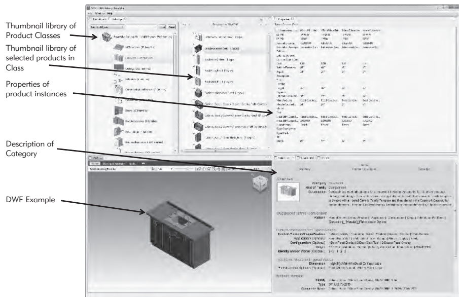
FIGURE 5–24 Multilevel structure of the SmartBIM Library. (Courtesy SMARTBIM LLC.)
