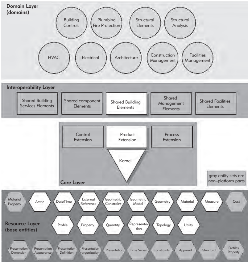
FIGURE 3-5 The system architecture of IFC subschemas.
