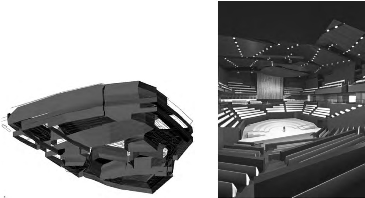
FIGURE 9-8-3 Computer building model of the concert hall shell, courtesy of Giencke and Company. This model was refined by Nagata, then fitted within the AutoCad Architecture model by LPR Architects. Integration is shown in the image on the right.
