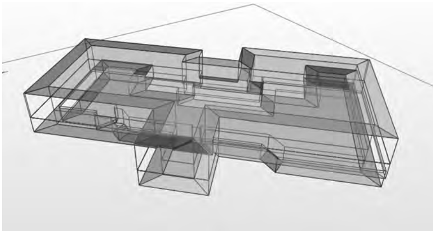
FIGURE 5-12 Example of perimeter and core thermal zone modeling.
