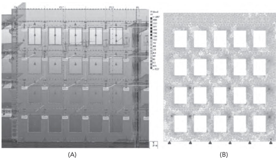
FIGURE 5–14 (A) A stack of lite-wall precast pieces in a Tekla Structures model with loads defined, and (B) the same section in the STAAD PRO finite element analysis package.
