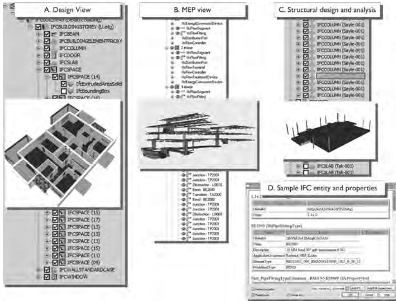
FIGURE 3-4 IFCs consist of a library of object and property definitions that can be used to represent a building project and support use of that building information for a particular purpose.
