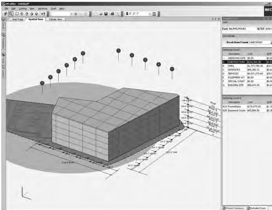
FIGURE 9-9-5 Screenshot of the DProfiler system, showing a 2D spatial view of the project, a 3D view, the related Proforma (left corner view), and cost details (along the right side).
